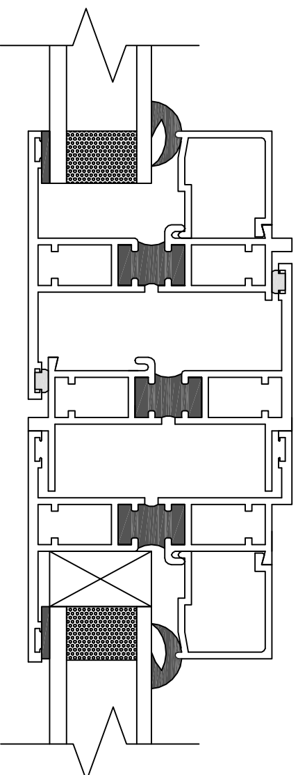
SECTION C
