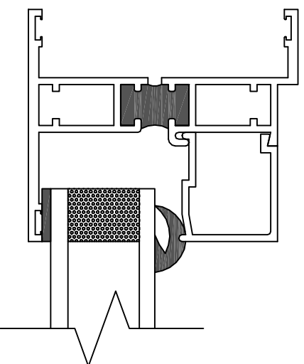
SECTION A
