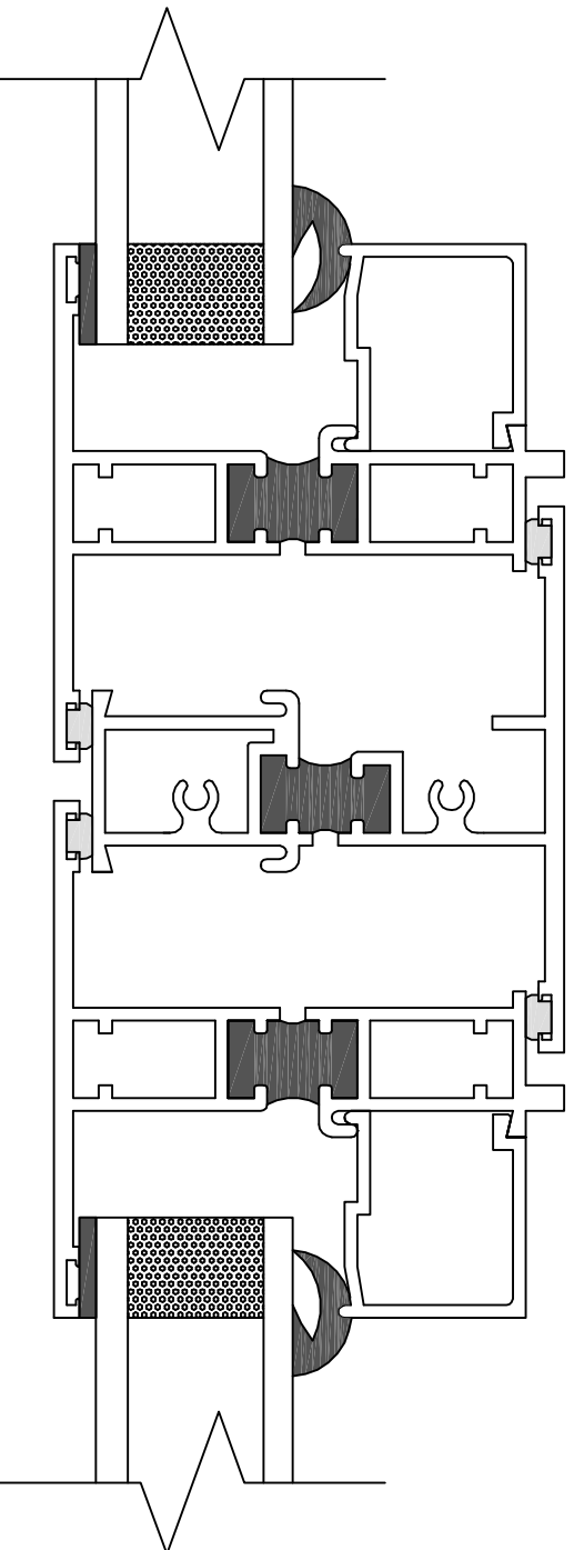
SECTION B
