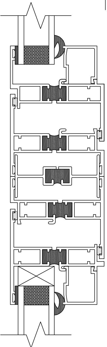
SECTION C
