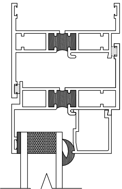
SECTION A
